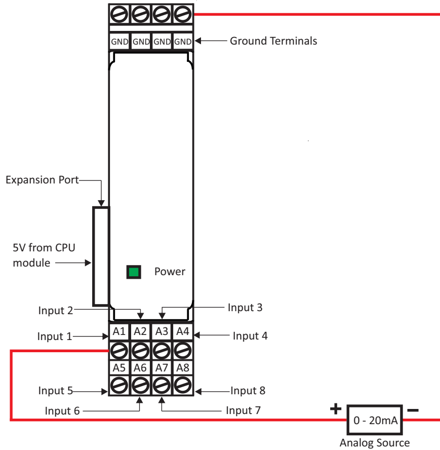
Figure 5: The wiring diagram of the Analog Input Module.
