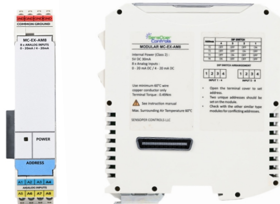
Figure 1: Front and Side view of Analog Input module
