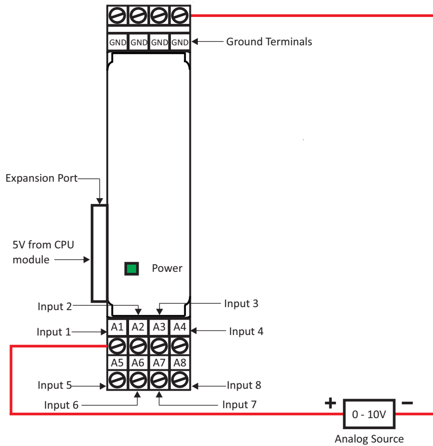
Figure 1(a): Analog Input Expansion module power up and Input terminals wiring.
